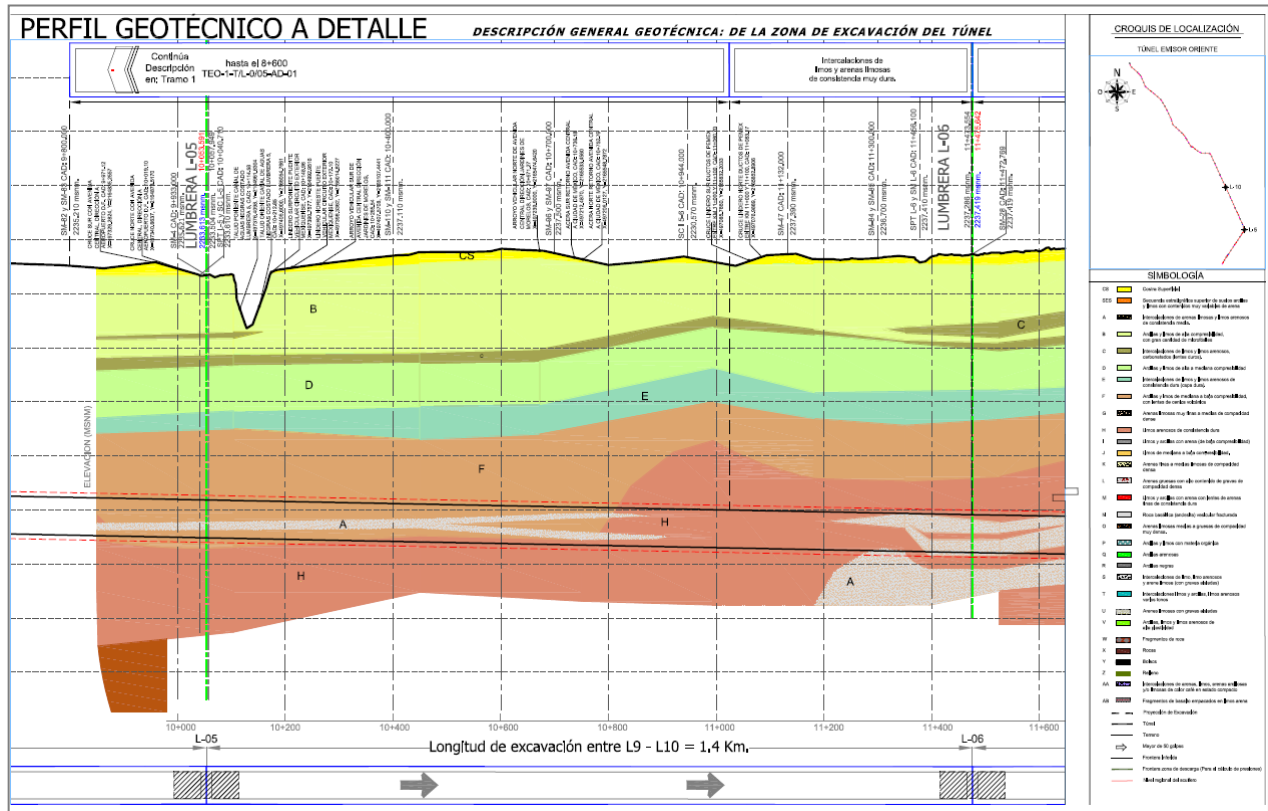
Figure 1. Geological profile of the tunnel between Shafts 5 and 6
